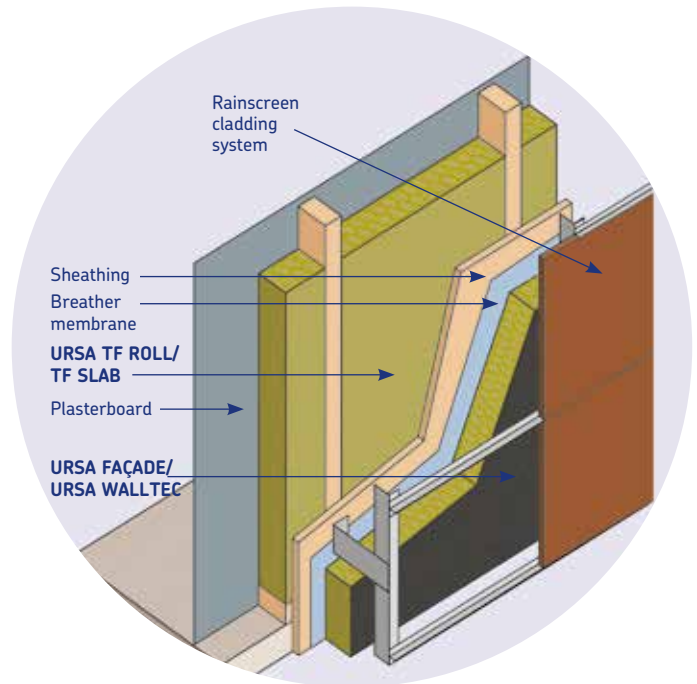
Figure 4 – Rainscreen Cladding on Timber Framed Wall
