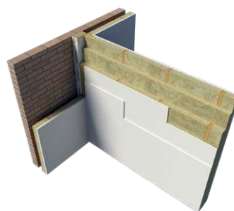
Figure 2 PWCB
