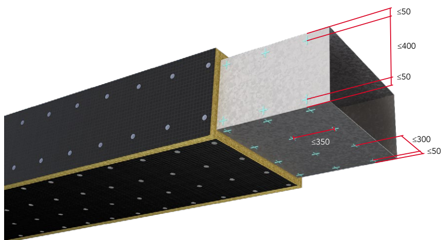
Figure 5 Horizontal duct
