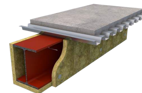
Figure 1 FIREPRO® BEAMCLAD® Systems
