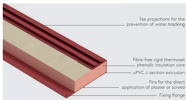
Figure 1: Kingspan Kooltherm® Cavity Closer
