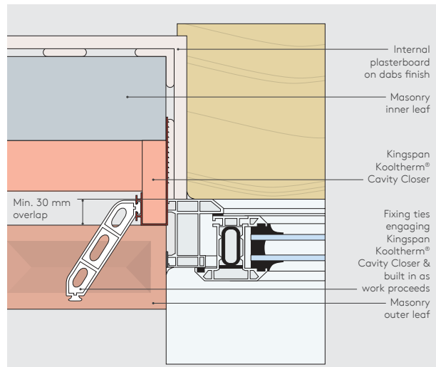
Figure 7: Jamb Detail Incorporating Kingspan Kooltherm® Cavity Closer at a Normal Reveal
